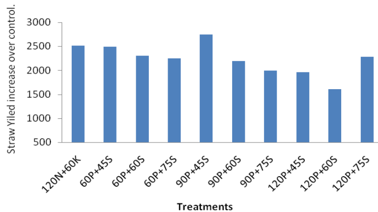
Figure 4: Straw yield increase over control by different levels of P and S
