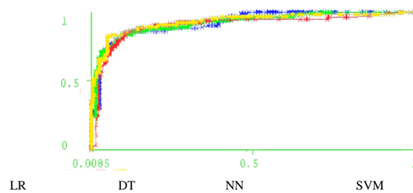
Fig 2. ROC curve
