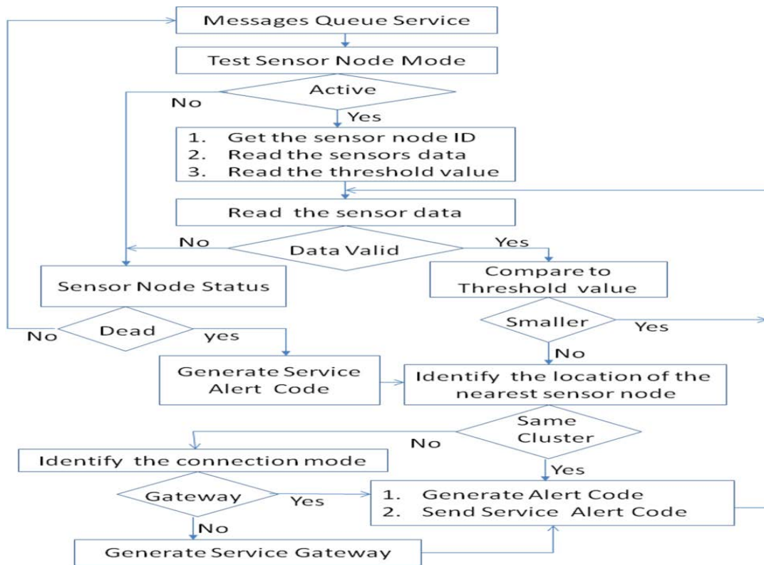
Figure 13: Message service structure.
