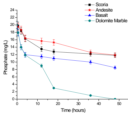
Figure 4: The phosphate removal trend of 20mg/L concentration at 25 0 C and shaking speed of 150rpm
