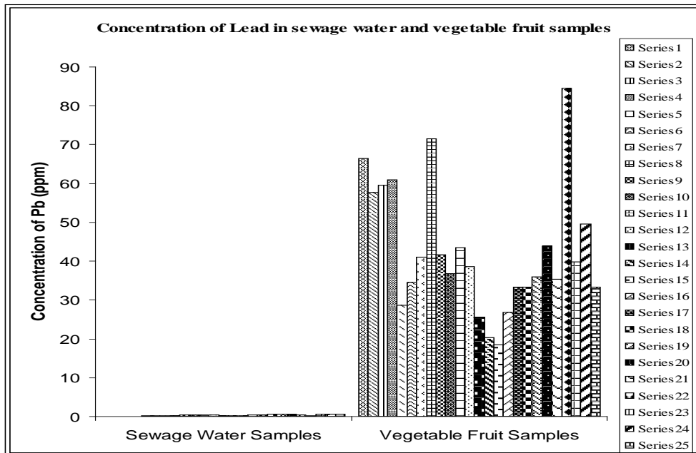
Fig 13: Pb concentration in Sewage water and vegetable fruit samples
