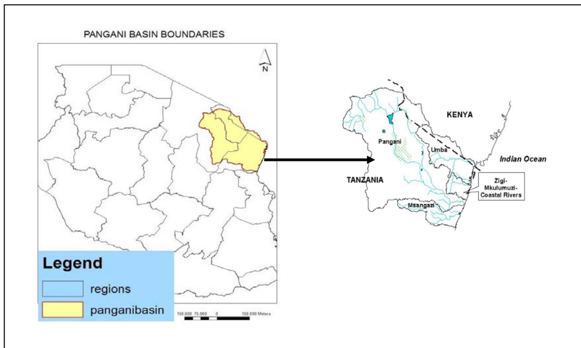
Figure 1: Pangani River Basin location in Tanzania and Boundaries [18].
