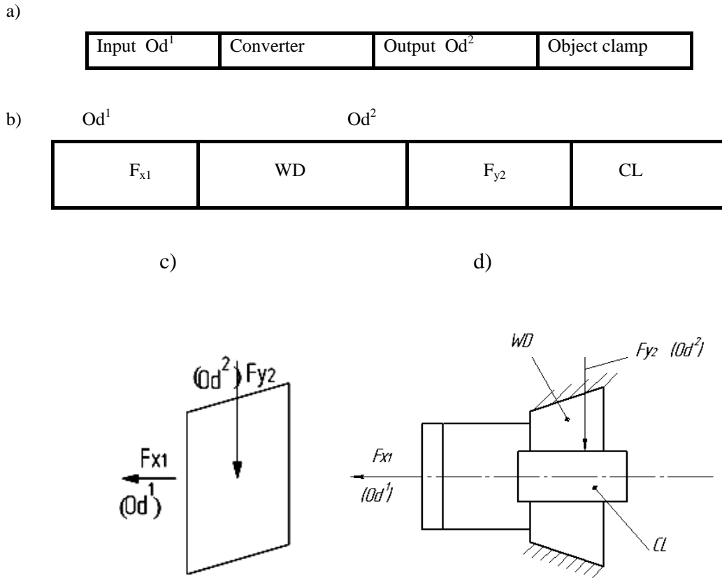
Fig. 5. The generalized structure of (a), a particular genetic formula (b), a power flow (c) and Scheme V, or the collet chuck (d)
