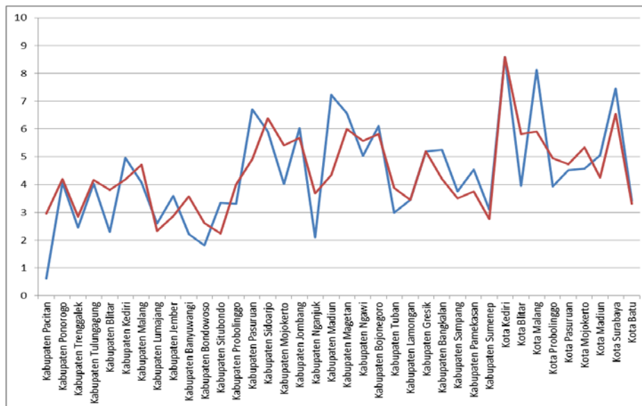
Figure 13: TPT distribution pattern with multivariable NGWR-TS model.
